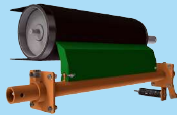
Head Scraper
