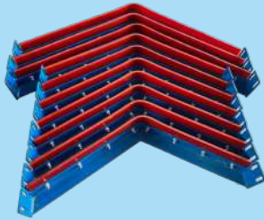
V-Scraper
